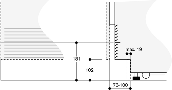
Base detail
